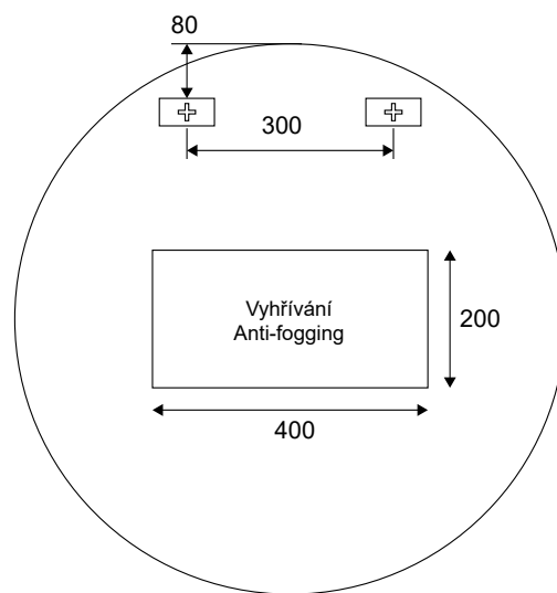
Pohled zezadu Rear view
